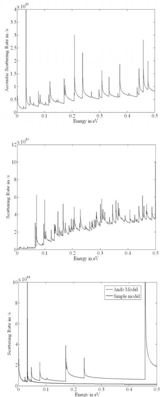
Figure 2: Acoustic phonon scattering rate as a function of energy for a 10nm wire for sheet density N_s \sim 10^{13}/\text{cm}^2 (top panel); Non-polar optical phonon scattering rate as a function of energy for a 10nm wire for sheet density N_s \sim 10^{13}/\text{cm}^2 (middle panel); Surface Roughness scattering rate as a function of energy for the two models considered (10nm wire for sheet density N_s \sim 10^{13}/\text{cm}^2 ) (bottom panel).
