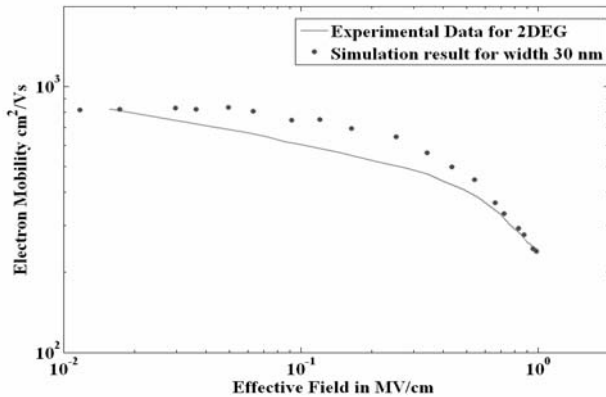
Figure 3. Electron mobility of a 30nm wide wire and 2-d electron gas.
