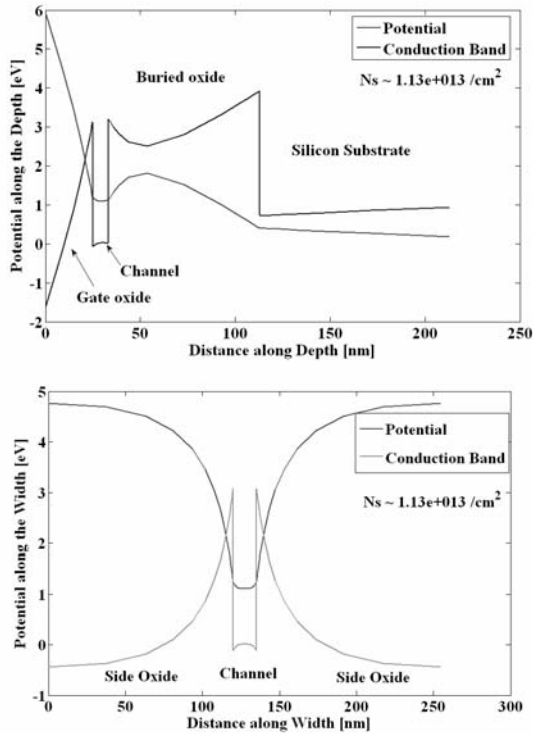
Figure 1: Confining potential profile along the depth (top panel) and width (bottom panel) of the wire.
