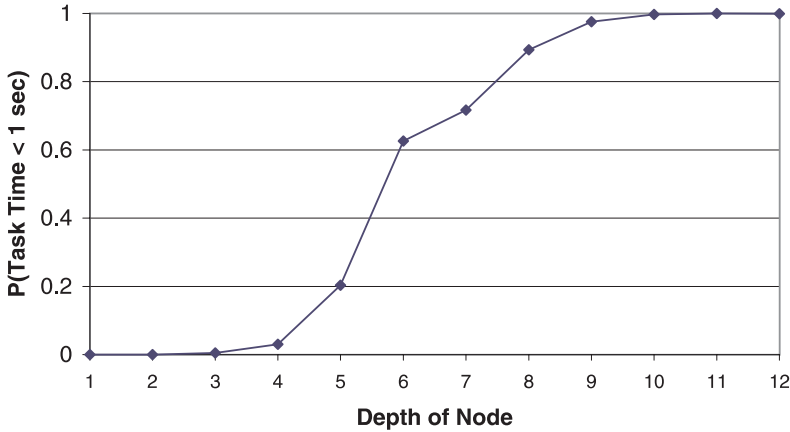
Fig. 5. Likelihood of fast tasks for nug25
