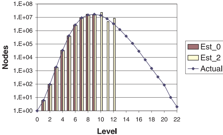
Fig. 1. Performance of estimator on nug25
