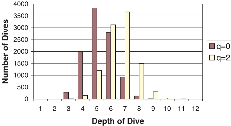
Fig. 2. Dive depths using estimator on nug25
