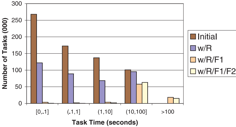
Fig. 4. Distribution of task times for MWQAP on nug25
