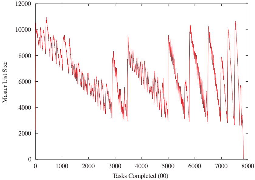
Fig. 7. Nodes in master queue during nug30 computation
