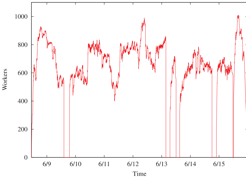
Fig. 6. Number of workers in nug30 computation
