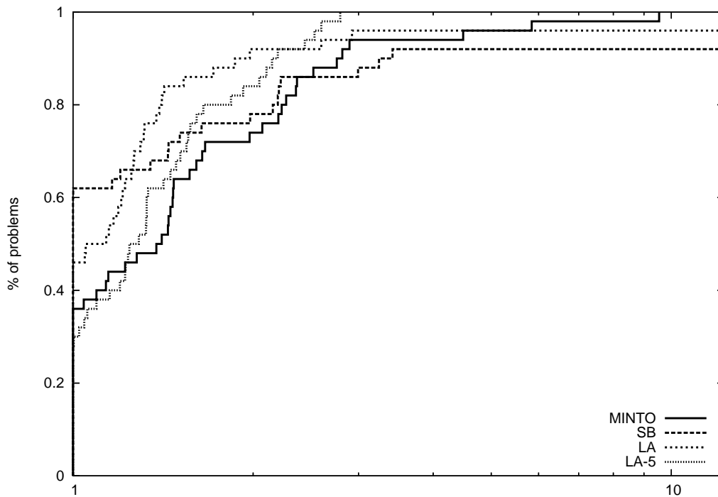
FIGURE 10. Performance Profile of Number of Evaluated Nodes
