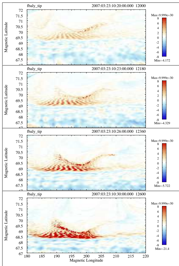
Figure 2. Ballooning modes mapped to the ionosphere. Field lines are traced from every location on the plot from the ionosphere through the magnetosphere. For field lines that are closed to color coding is according to the same force imbalance shown in Figure 1 at the tip of the field line. The pattern seen is the expected pattern of ionospheric emissions caused by the ballooning mode. However, no statement about the luminosity can be made because we do not know the mechanism that would cause the aurora.
